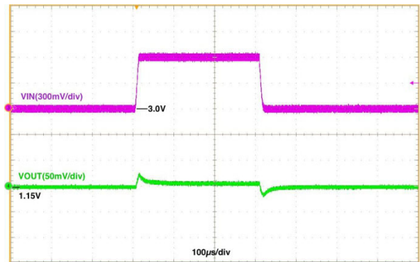
Figure 12. Line Transient, V_{IN} = 3.0\text{ V} \leftrightarrow 3.6\text{ V} , T_R = T_F = 10\text{ µs} , I_{OUT} = 500\text{ mA}
