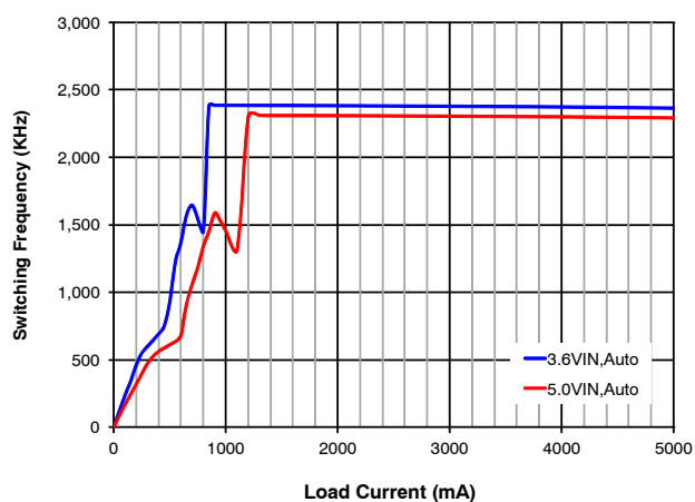
Figure 8. Frequency vs. Load Current
