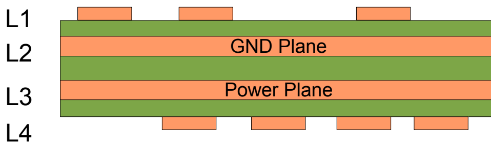
Figure 68: Four-Layer Stack-up
