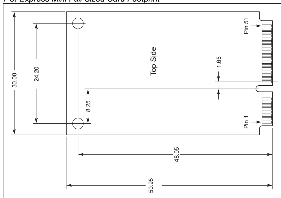
Figure 11: PCI Express Mini Full Sized Card Footprint
