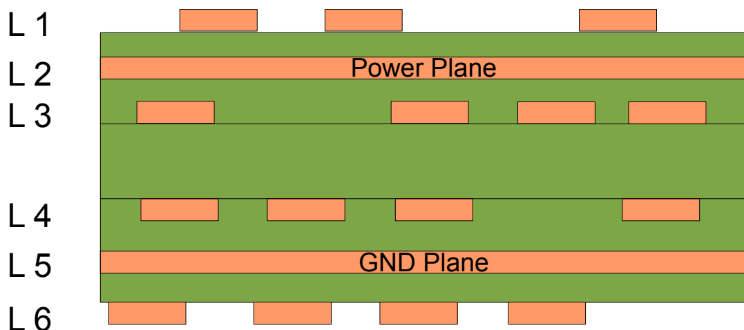
Figure 69: Six-Layer Stack-up
