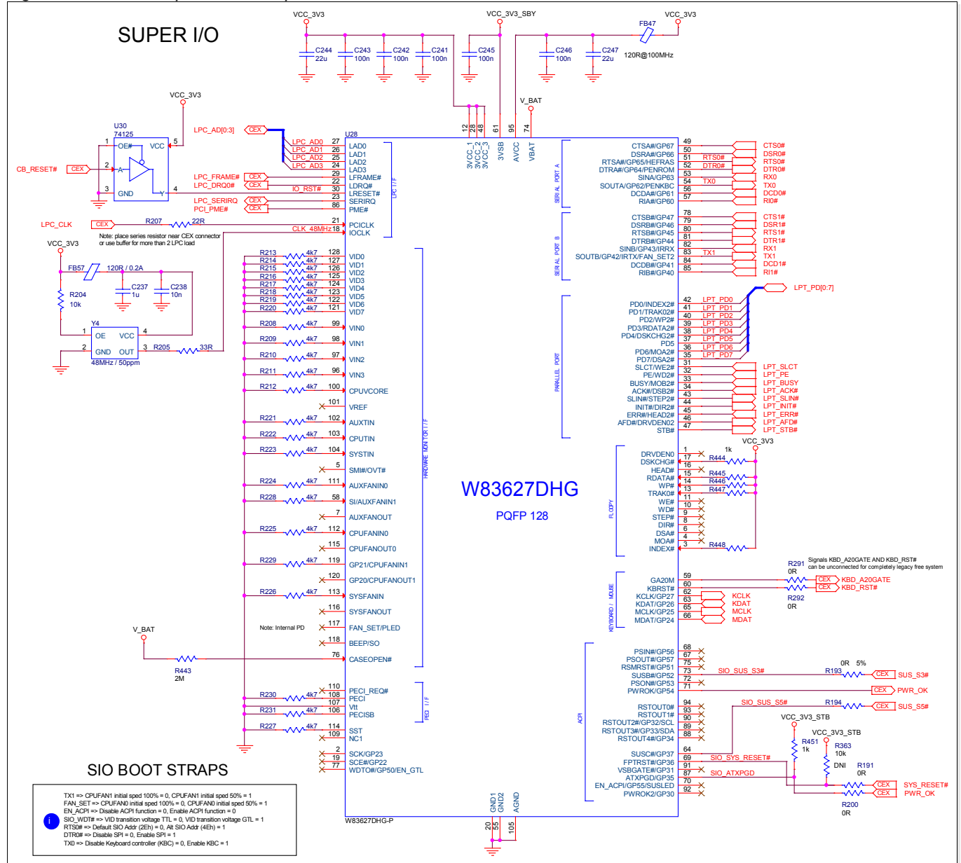
Figure 44: LPC Super I/O Example
