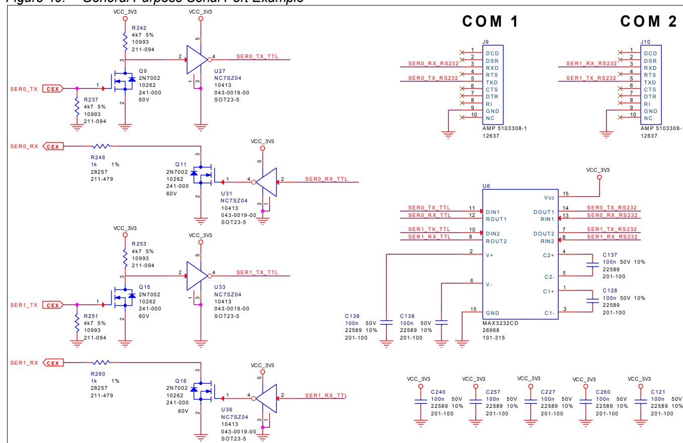
Figure 49: General Purpose Serial Port Example
