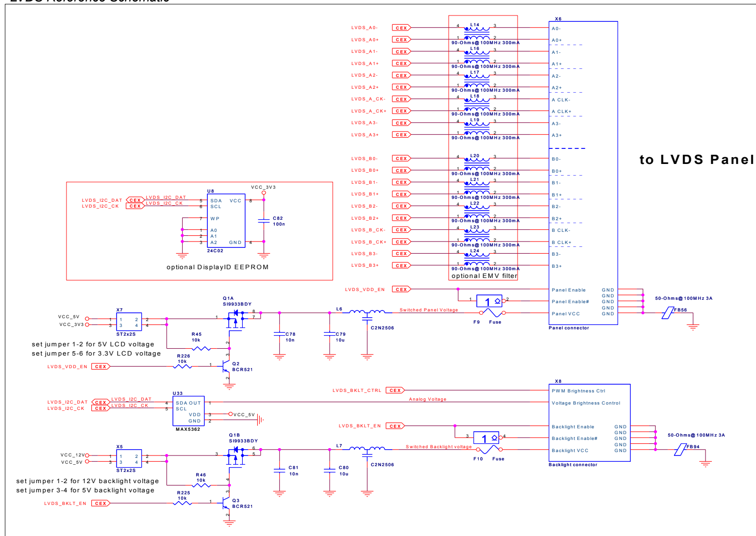
Figure 34: LVDS Reference Schematic
