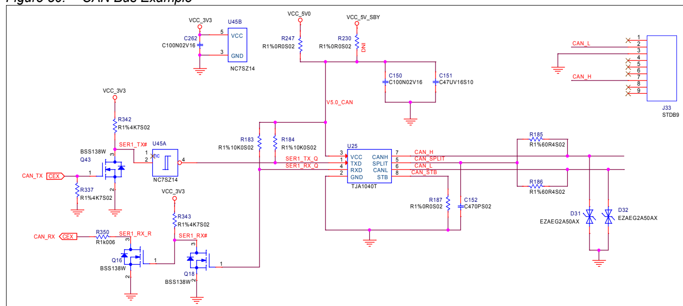
Figure 50: CAN Bus Example
