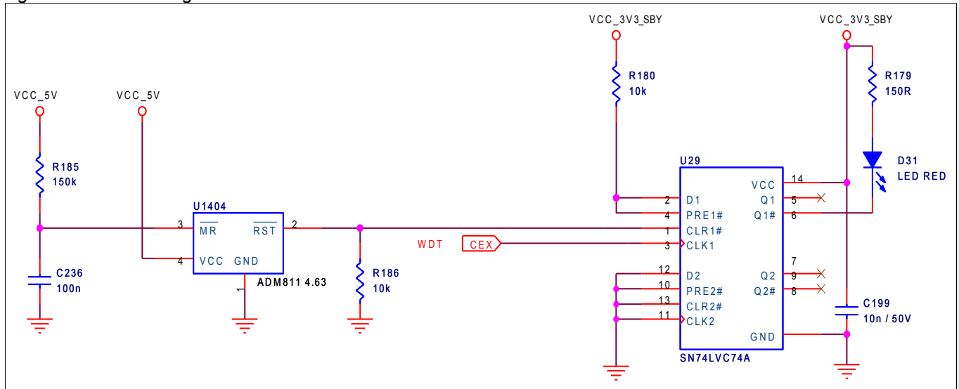
Figure 54: Watchdog Timer Event Latch Schematic
