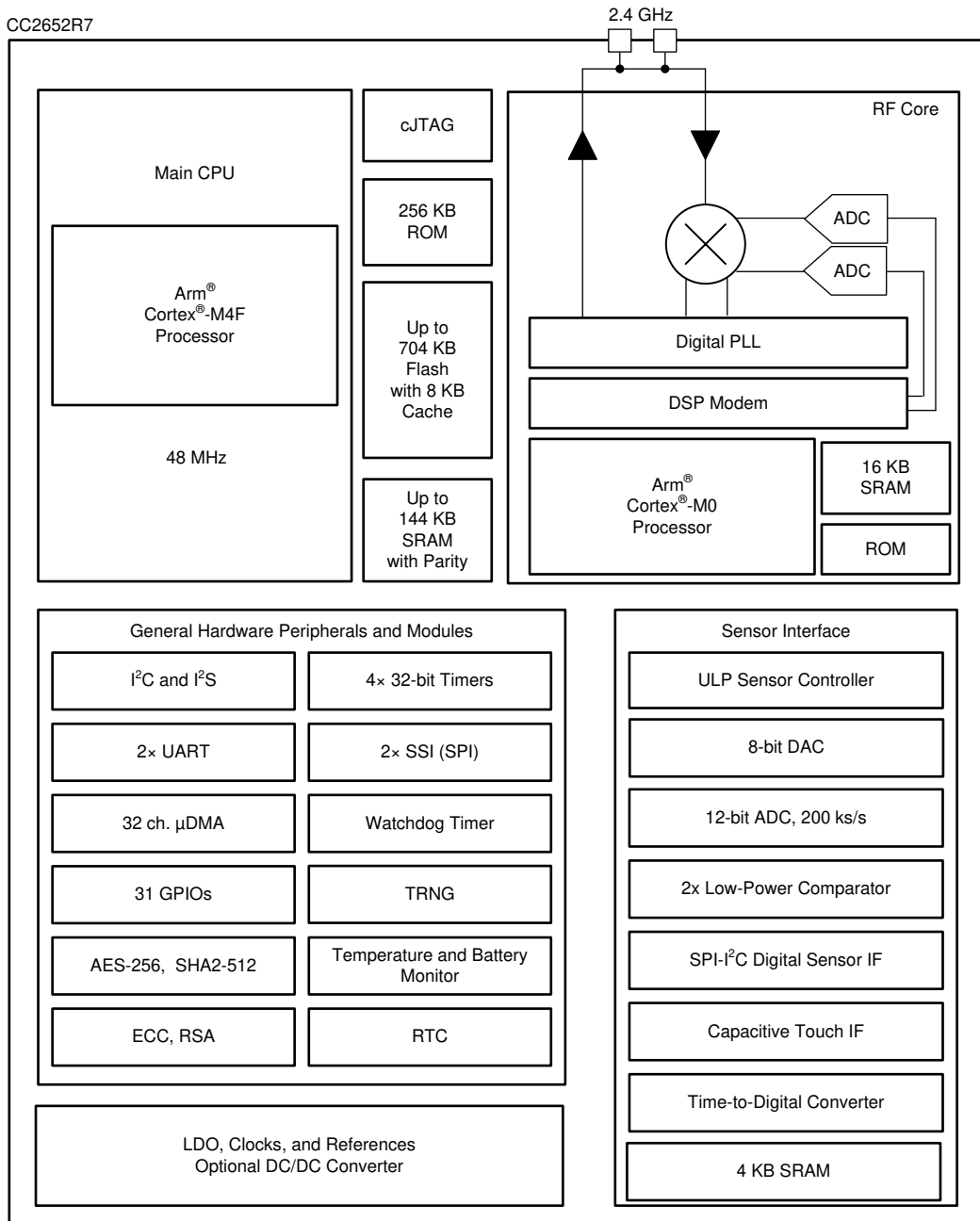
Figure 3-1. CC2652R7 Block Diagram
