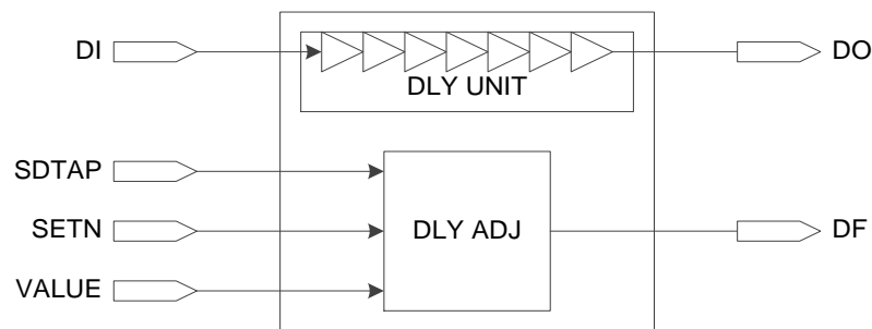
Figure 3-8 IODELAY
