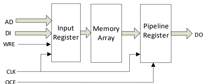
Figure 3-25 Pipeline Mode in Single Port, Dual Port and Semi-Dual Port
