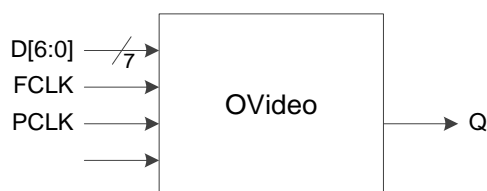
Figure 3-18 I/O Logic in OVideo Mode
