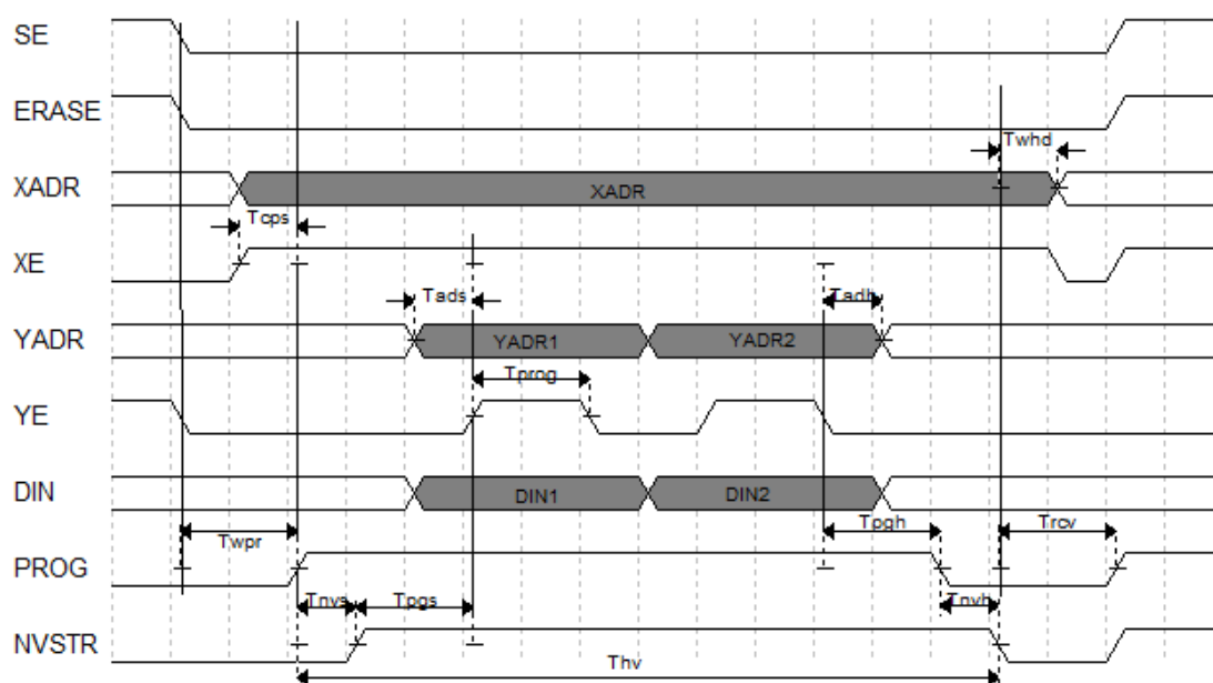
Figure 4-2 User Flash Program Operation
