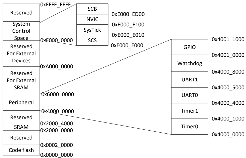
Figure 3-34 Memory Mapping
