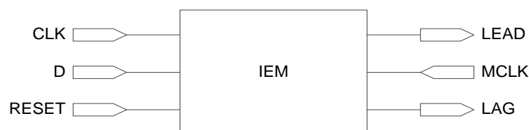
Figure 3-10 IEM Structure
