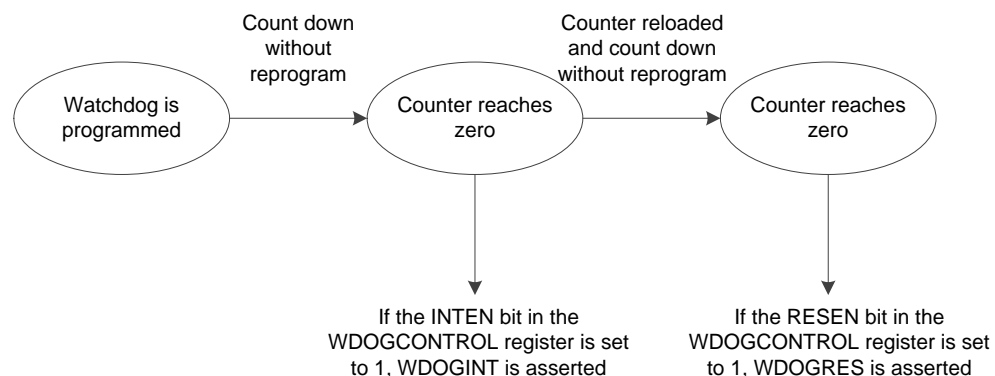
Figure 3-33 Watchdog Operation
