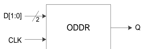
Figure 3-14 I/O Logic in DDR Output Mode
