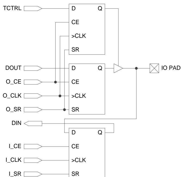
Figure 3-12 I/O Logic in SDR Mode
