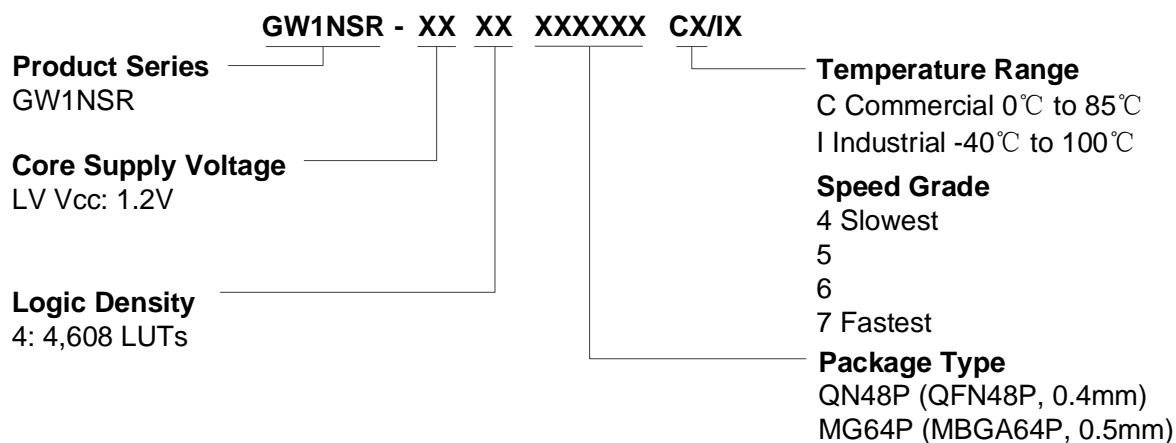
Figure 5-3 GW1NSR-4 Part Naming - Production
