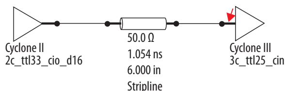
Figure 6: Terminator Wizard Results From HyperLynx Simulation Software by Mentor Graphics Corporation
