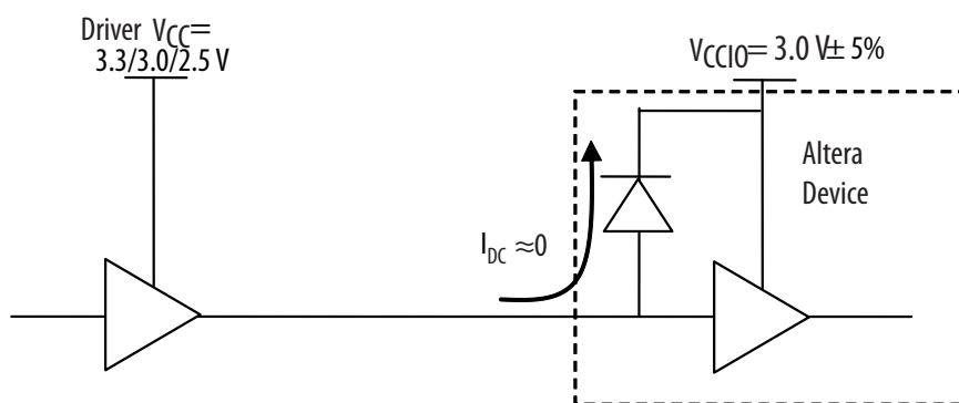
Figure 10: Supported Altera Device Input Setup with 3.0 V V_{CCIO}
