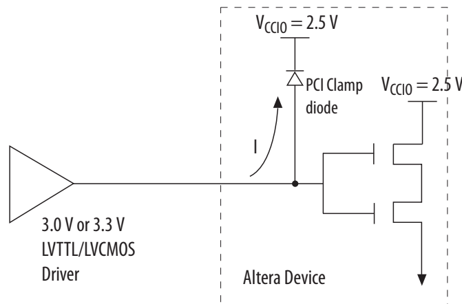
Figure 2: PCI Clamp Diode in Supported Altera Devices
