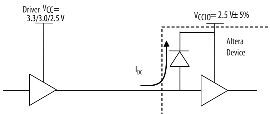
Figure 9: Supported Altera Device Input Setup with 2.5 V V_{CCIO}
