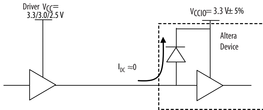
Figure 11: Supported Altera Device Input Setup with 3.3 V V_{CCIO}
