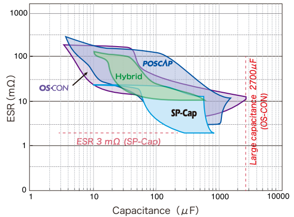
Capacitance vs. ESR
