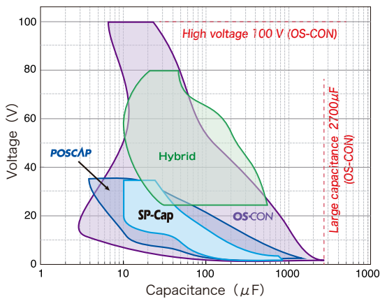
Voltage vs. Capacitance
